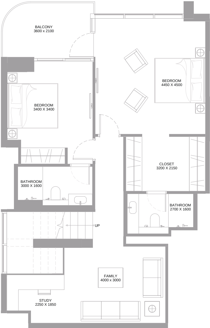
LOWER LEVEL
